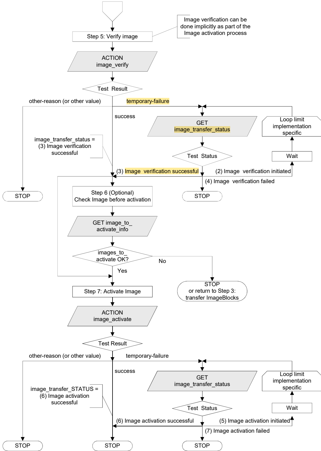
Figure 11 – Image transfer process flow chart
